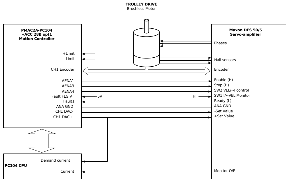
Figure 2: PMAC arrangement for control of the trolley drive.
