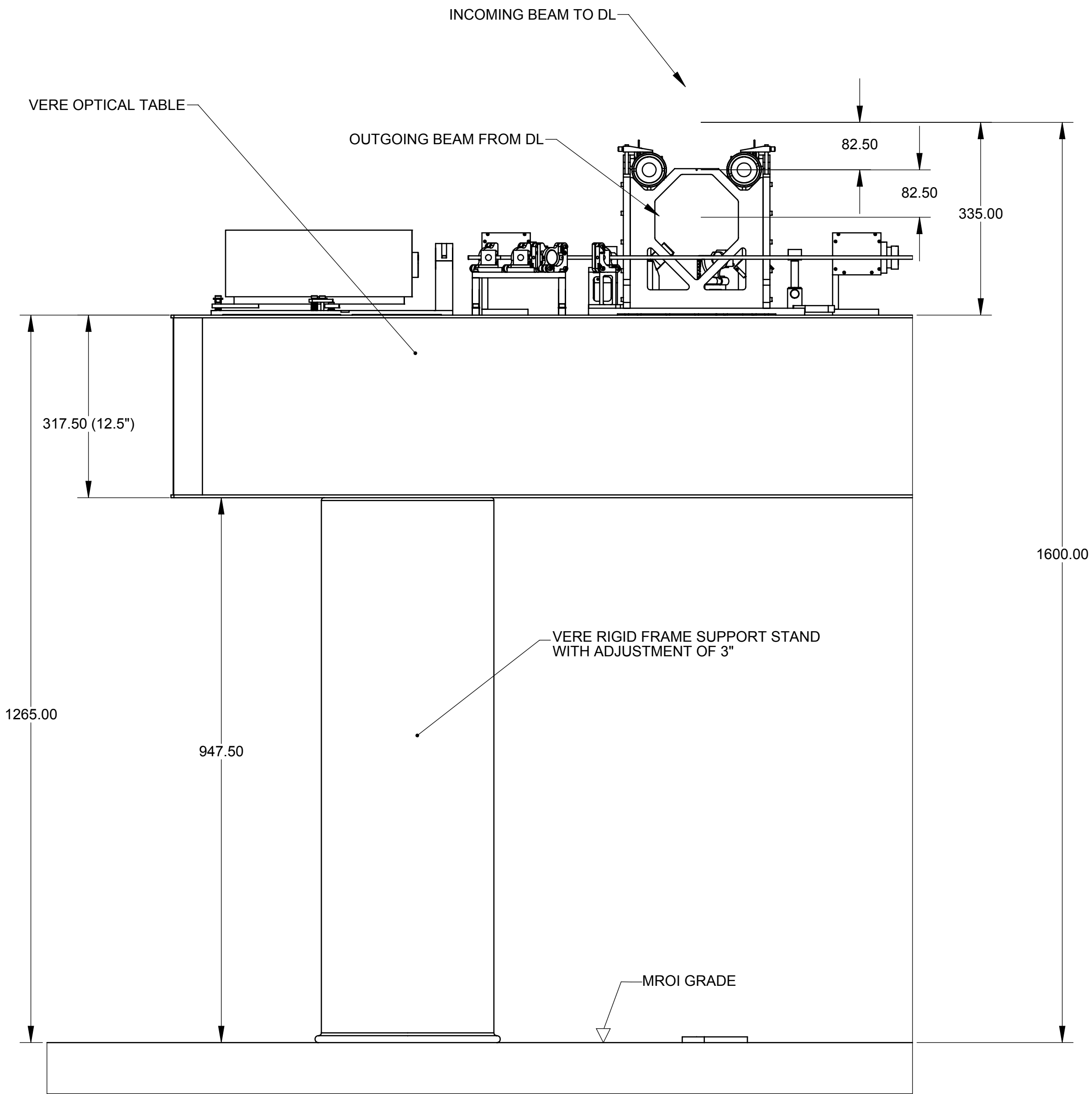
SIDE VIEW OF OPTICAL TABLE
