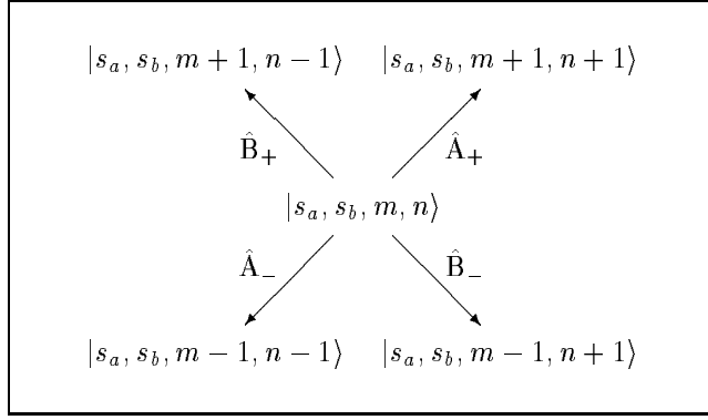
Figure 1: Raising and Lowering Operators for Spin- s Irreducible Representation of the Lorentz Group.
